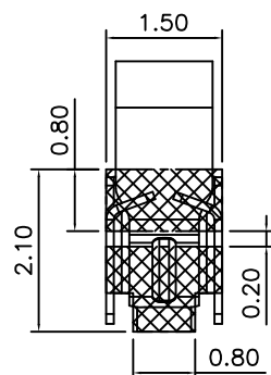
RECOMMENDED PCB LAYOUT TOLERANCE ±0.05 (焊盘推荐图)
