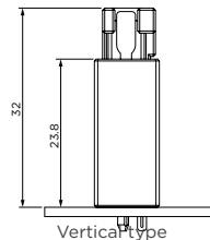
Vertical type
