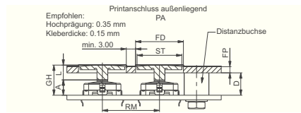
THT terminal outward
