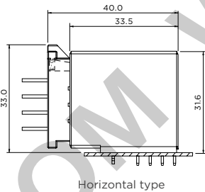
Horizontal type
