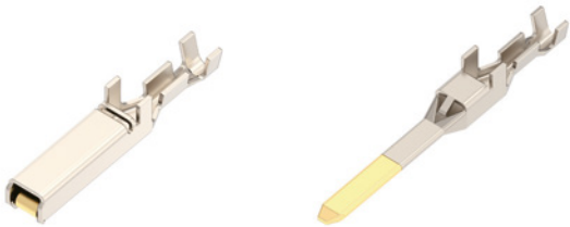
Receptacle Contact (used in receptacle housing)
