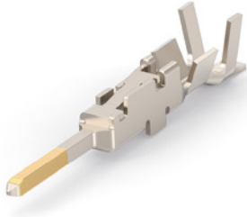
Tab contact (for Tab housing)
