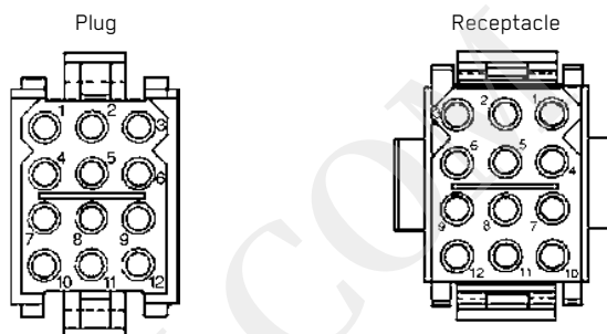
12-way
