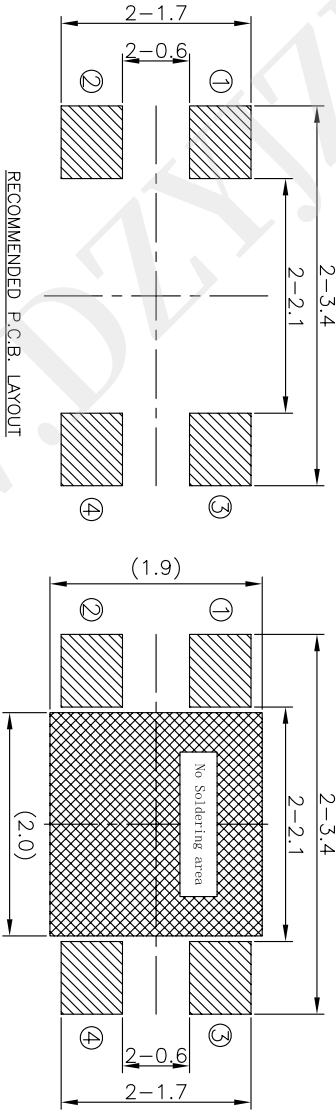
LAND PATTERN PLAN
