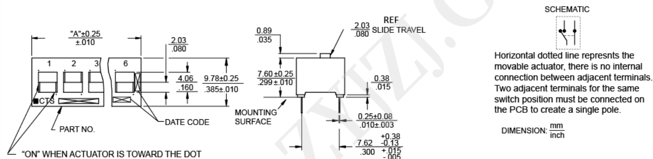
Figure 2 – SPDT
