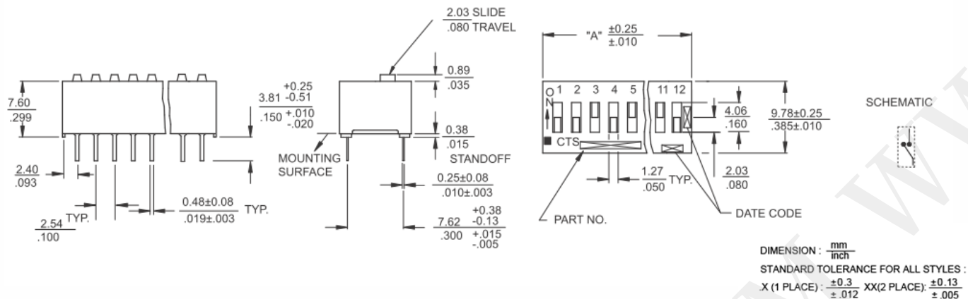
Figure 1 - SPST
