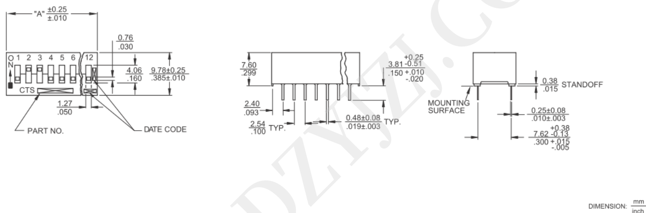
Figure 3 – Extended Actuators
