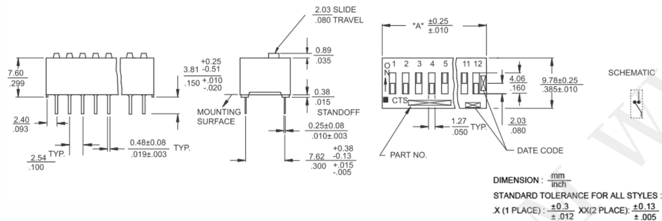
Figure 1 - SPST
