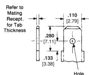
Mating 110 Series Tab Dimensions Type 3
