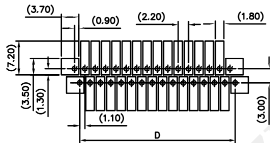
METAL MASK DIMENSIONS(REF.) MASK THICKNESS T=0.15mm
