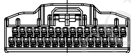
2*16PIN
