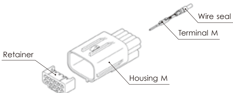
Connector M
