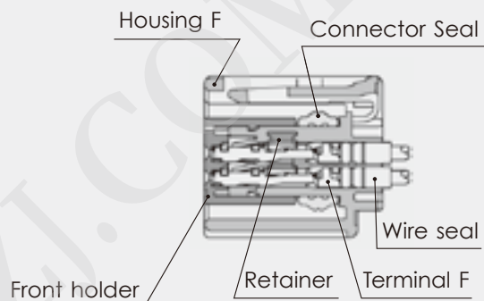
Connector F
