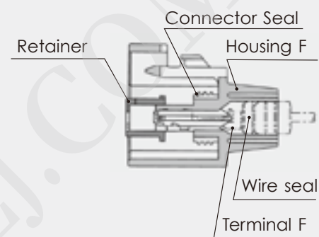
Connector F
