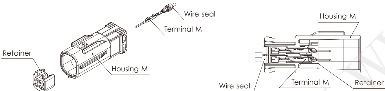
Connector M
