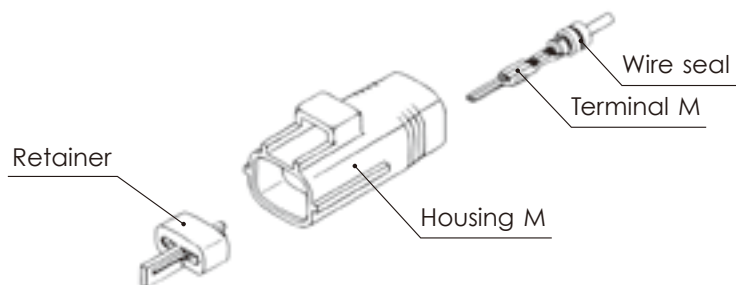
Connector M
