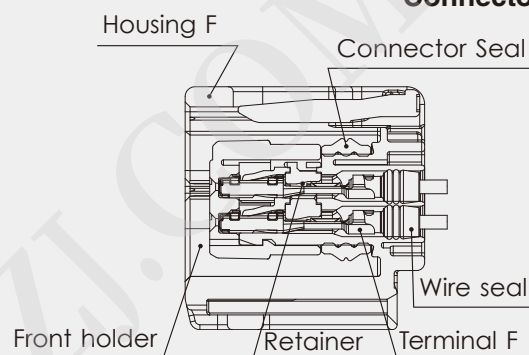
Connector F
