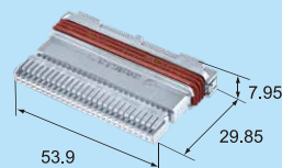
F (6189-8468) 灰 52Way-Inner-ASSY-2
