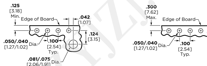
Recommended Mounting Hole Pattern for .062 [1.57] Thk. PC Board (Solder Side of Board Shown)
