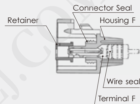
Connector F
