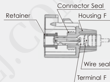
Connector F
