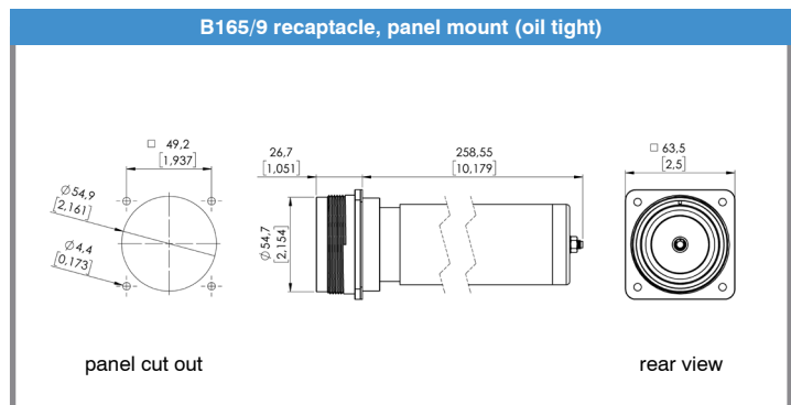
B 165/9 receptacle, panel mount
