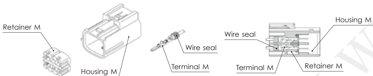
Connector M
