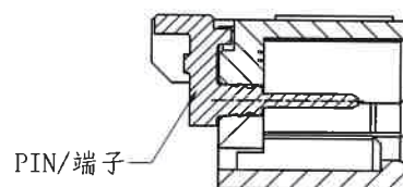
SECT: E-E
