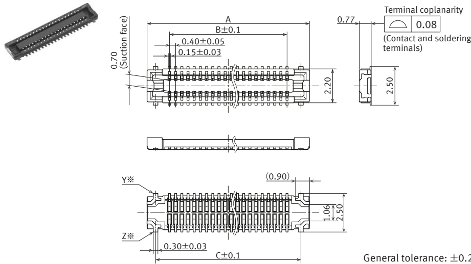
External dimensions
