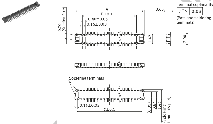
External dimensions
