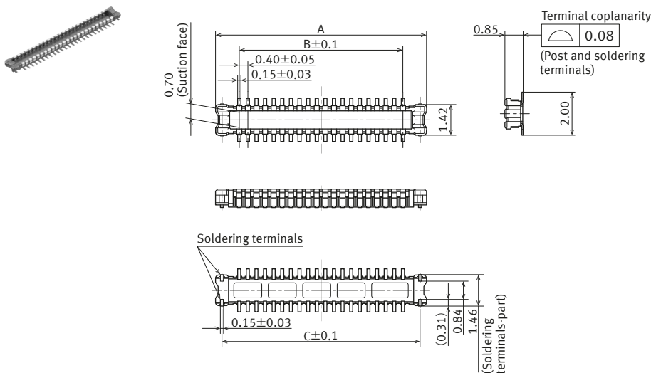
External dimensions
