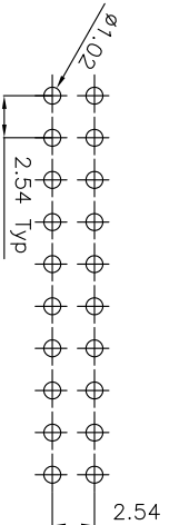
RECOMMENDED PCB LAYOUT (TOLERANCE:±0.10)
