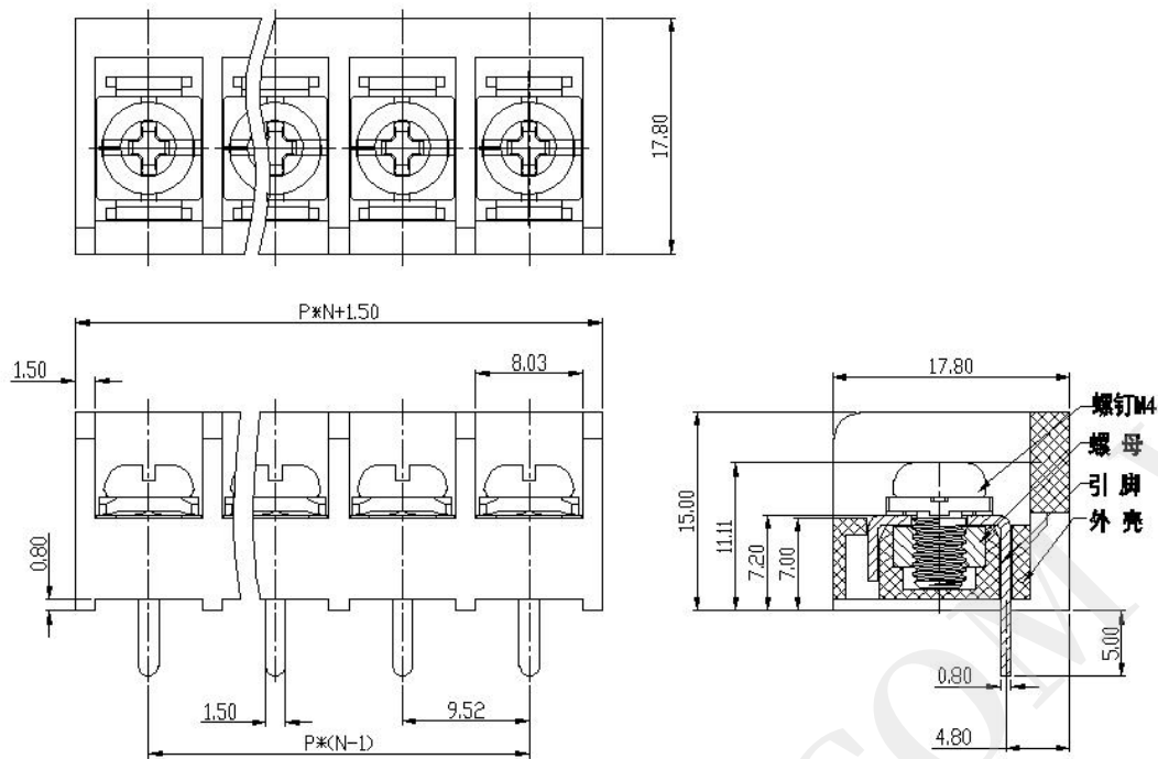
外形尺寸 (Shape Dimension)
