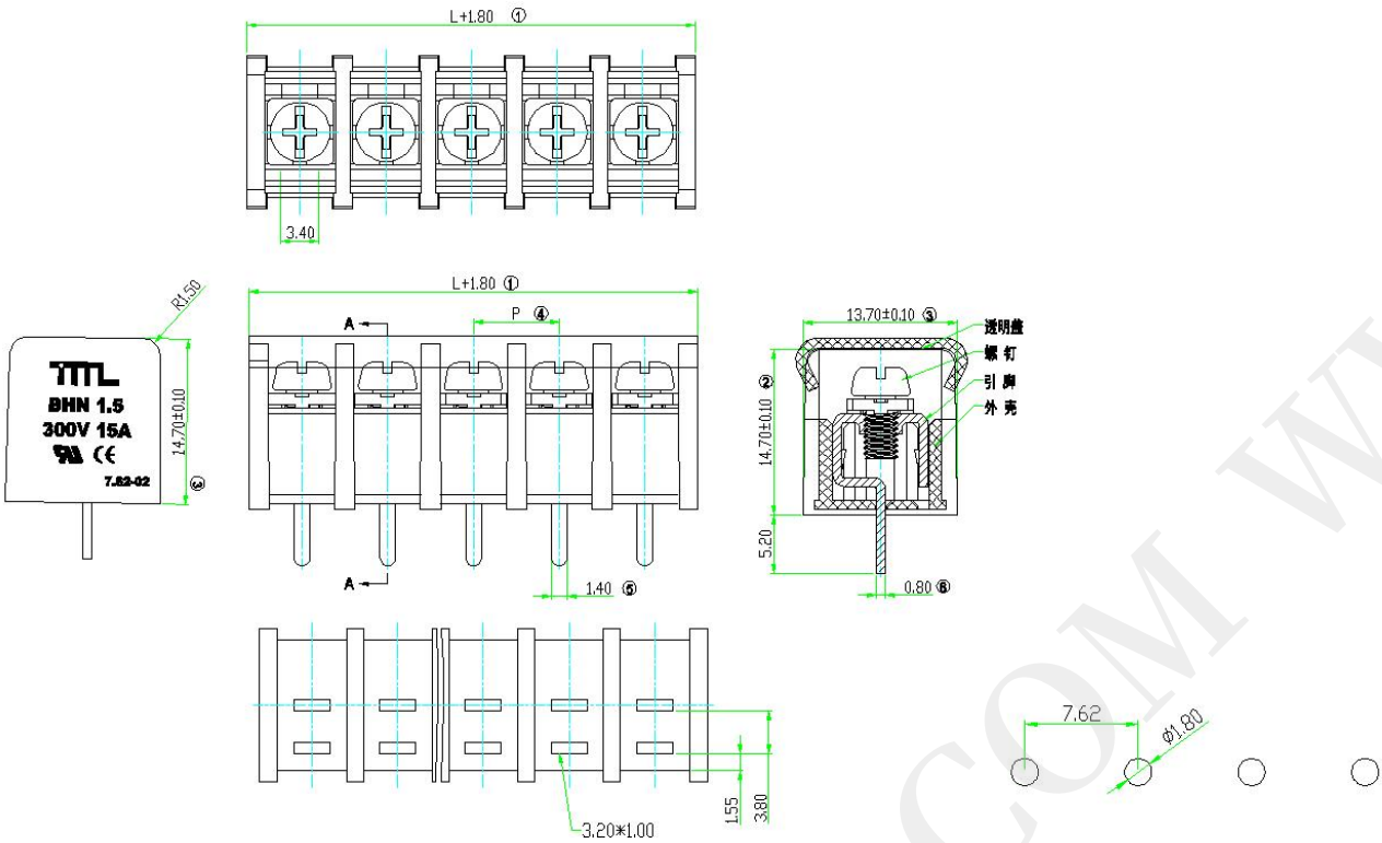
外形尺寸 (Shape Dimension)
