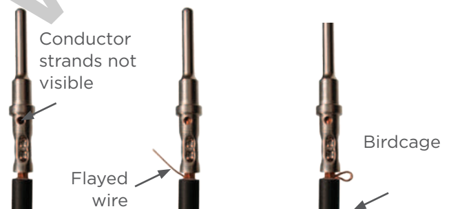
Unacceptable Crimps
