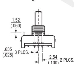
BUSHING MOUNTED - HOUSING H
