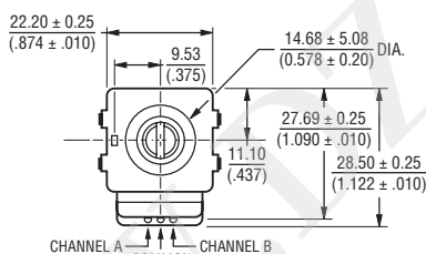
Shaft Style C
