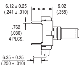
SNAP-IN MOUNT - Housing G
