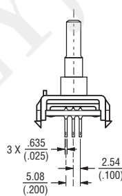
Shaft Style R
