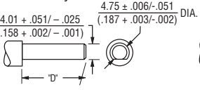
Shaft Style J
