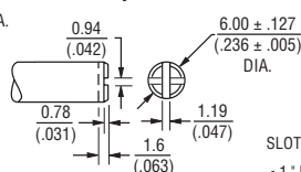
Shaft Style R
