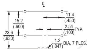
PCB MOUNTING DIMENSIONS (Housing Styles B and E)
