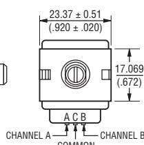
PCB BRACKET MOUNTED - HOUSING B Dimensions not given are the same as Bushing Mounted.
