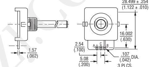
PCB MOUNTING DIMENSIONS
