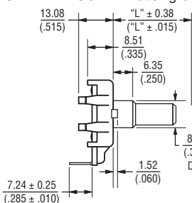
Shaft Style B
