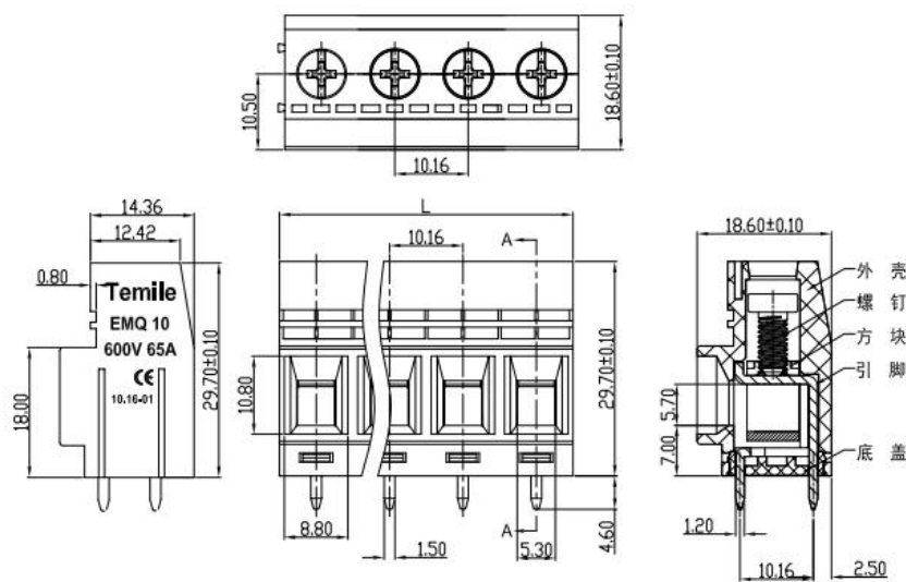
外形尺寸 (Shape Dimension)
