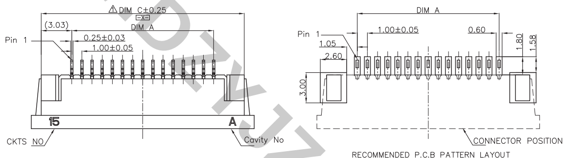
RECOMMENDED P.C.B PATTERN LAYOUT
