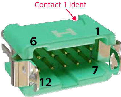
Male PCB mounted
