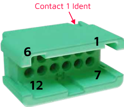
Male Crimp Housing
