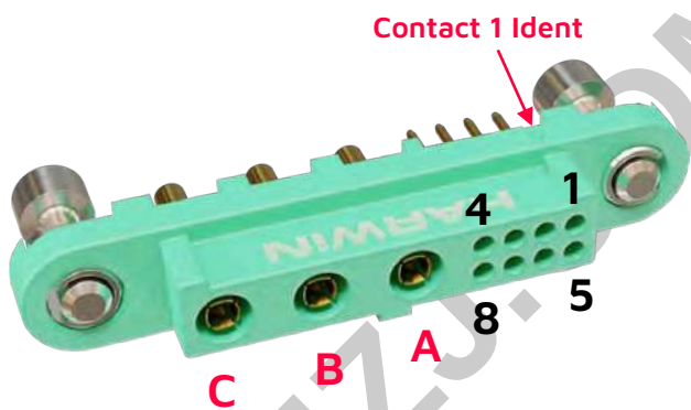
Female PCB mounted
