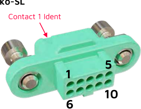
Female Crimp Housing
