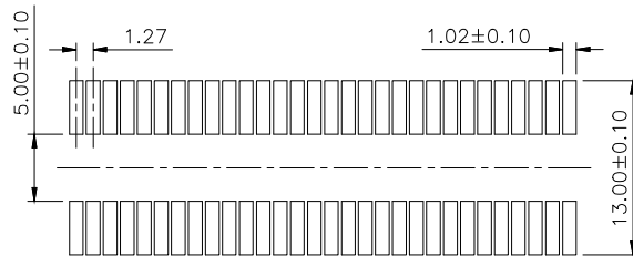
Recommended P.C.B. Layout(Top View) P.C.B. Thickness:1.2mm~1.6mm
