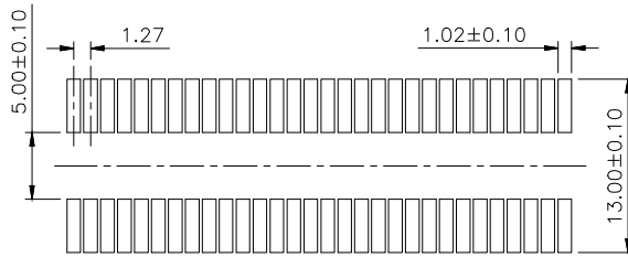
Recommended P.C.B. Layout(Top View) P.C.B. Thickness:1.2mm~1.6mm
