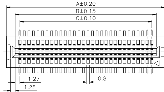
Recommended P.C.B. Layout(Top View) P.C.B. Thickness:1.2mm~1.6mm
