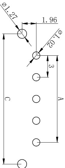
安装尺寸 MOUNTING MEASUREMENT
