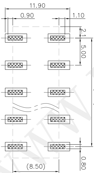
PCB LAYOUT
