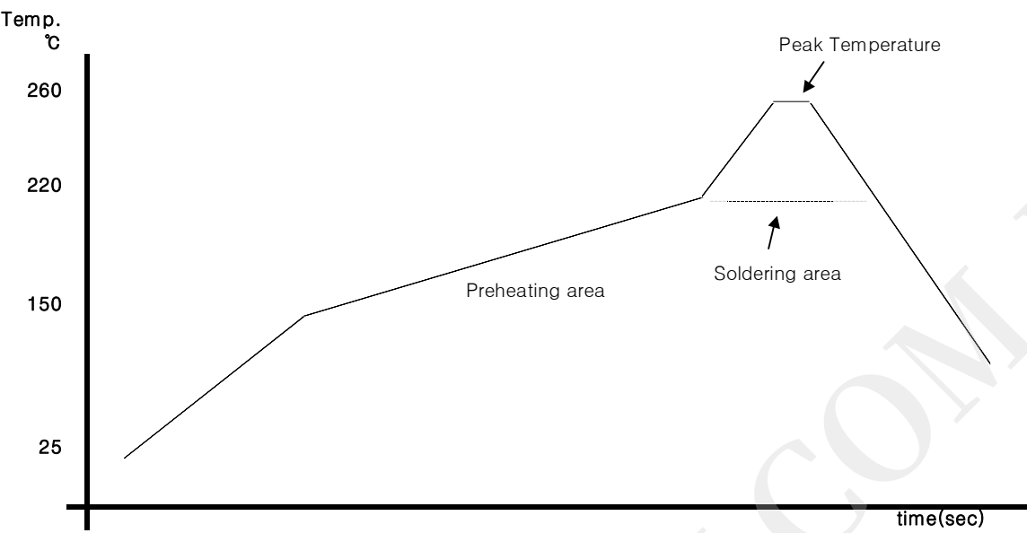
< Temperature profile >
