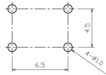
P.C.B MOUNTING HOLE DIMENSION
