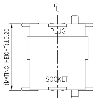
MATING HEIGHT SCALE:1.25:1
