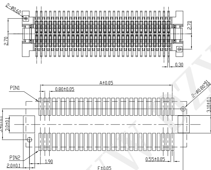
Recommended PC board pattern (TOP VIEW)
