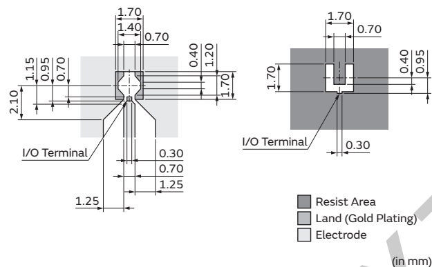
Standard Pattern Dimensions
