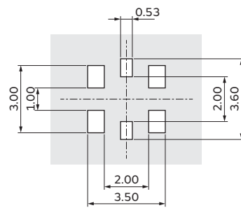
Standard Stencil Mask Pattern
