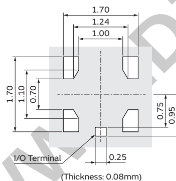
Standard Stencil Mask Pattern
