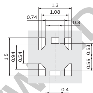
Standard Stencil Mask Pattern
