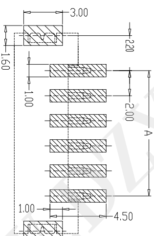
PCB LAYOUT TOLERANCE ±0.05
