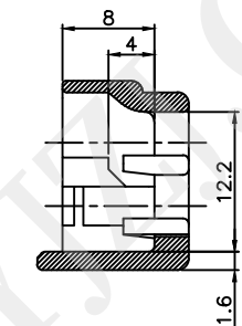
SECTION B-B(2/1)
