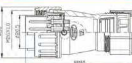
PLS-24◆-WGPM3 X-R
