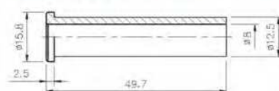
PLS-24◆-ADGM-R
