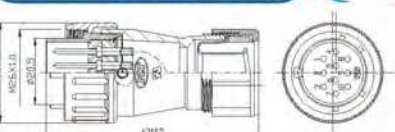
PLS-24◆-GPM3 X-R
