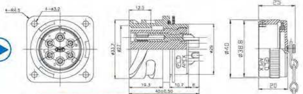
PLT3102A 20-15SA
