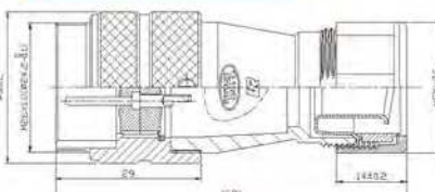
PLS-24◆-ADGM-R
