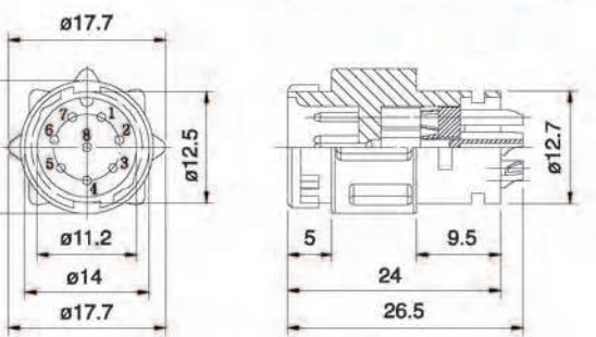
WPM16C12-8P-R
