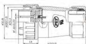
PLS-28-GPM4 X-R
