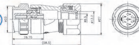
WPM-20-ADM-R
