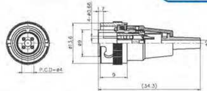
WPM-94-PM-R
