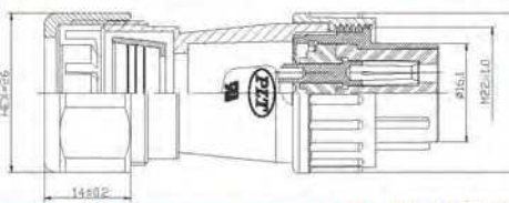
PLS-20◆-WGPF3 X-R
