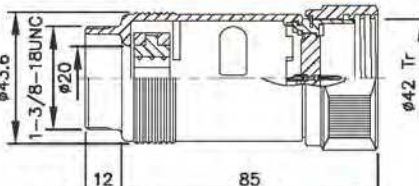
PLS-42◆-PM1
