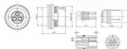
WPM-223-RF-R
