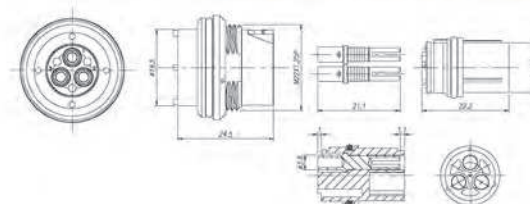
WPM-223-RFA-R
