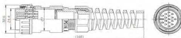
PLS-28-PMCG-R
