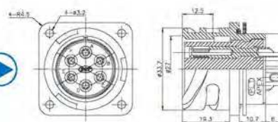
PLT3102A 20-15SA
