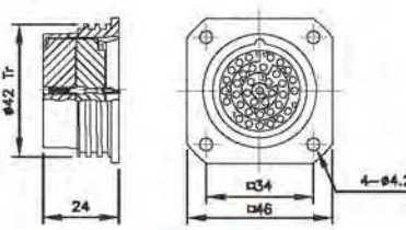
PLS-42◆-RF
