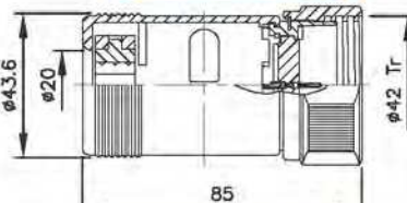
PLS-42◆-PM
