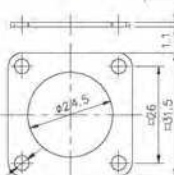
PLS-24C-RCaC-R
