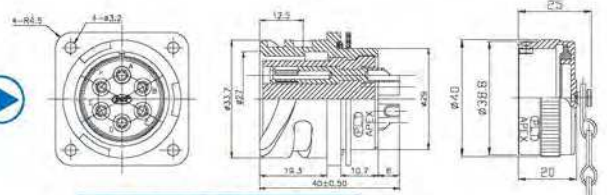
PLT3102A 20-15SA
