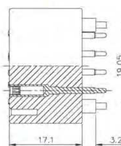
PLS-2710-PF
