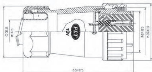
PLS-28◆-GPF X-R
