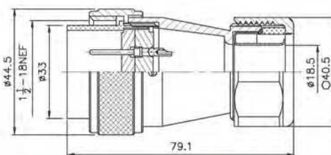
PLS-35 ◆ -GPM6-R 6=轉接3/4"軟管 Connected with 3/4" conduit
