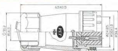
PLS-28◆-GPF4 X-R 4=轉接1/2"軟管 Connected with 1/2" conduit
