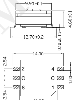
Solder pad layout as viewed from the top of the switch
