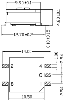
Solder pad layout as viewed from the top of the switch
