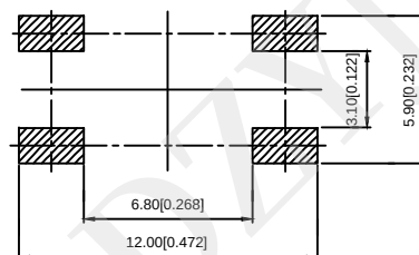
P.C.B MOUNTING HOLES
