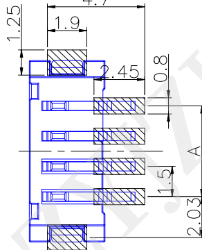
PCB. 焊接图 PCB. WELDING DRAWING
