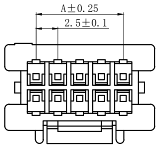
2X2-2X8PIN
