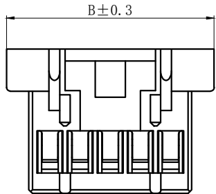
2X2-2X8PIN
