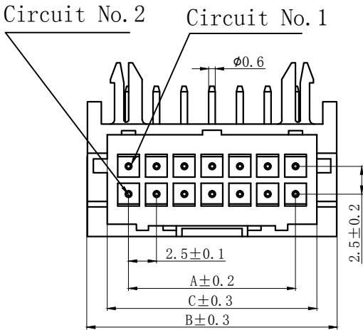
4-16PIN
